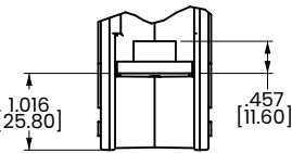
3/8-16 THREADED STUD CODE 2
