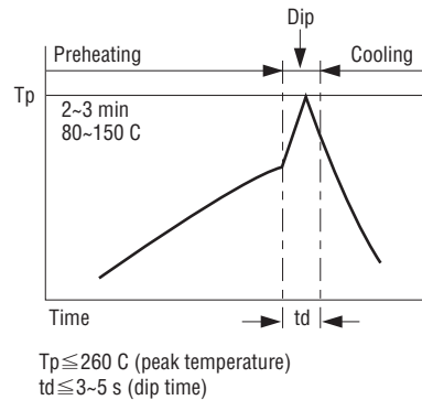
Recommended profile for lead-free soldering
