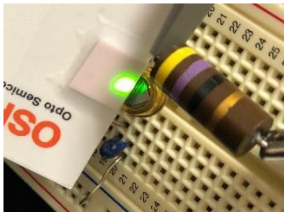
Figure 6: The sensor should be placed in the focused laser beam region.
