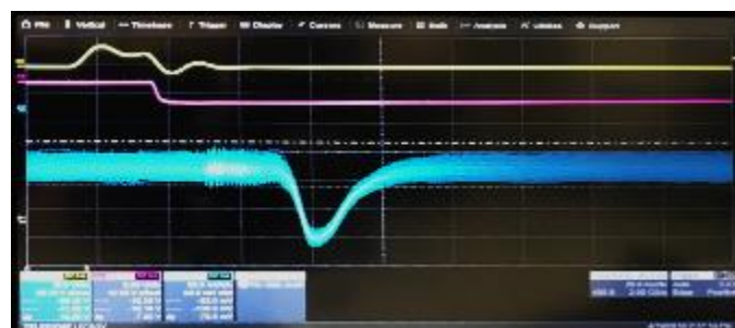
Figure 11: Three TOF flight measurements. The top panel shows a target 12" from the laser reflecting back into the sensor. The middle shows the laser reflecting from a target.
