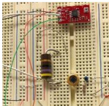
Figure 5: The Marktech APD is preceded by an RC filter and the output is measured across a low impedance, high wattage 47 Ohm resistor.
