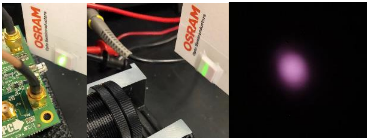
Fig. 4: Ensure that the frequency of the pulses are high enough that the laser can be observed using an infrared detector card (left) without the lens. Now focus the laser through the lens on the IR card as shown
