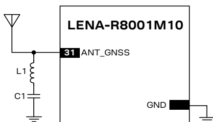
Figure 42: Simple notch filter for improved in-band jamming immunity against a single jamming frequency
