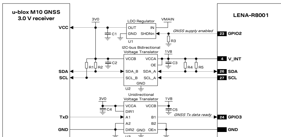
Figure 59: Application circuit for connecting LENA-R8001 modules to u-blox 3.0 V GNSS receivers
