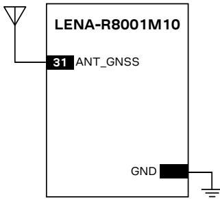
Figure 38: Minimum circuit with GNSS passive antenna
