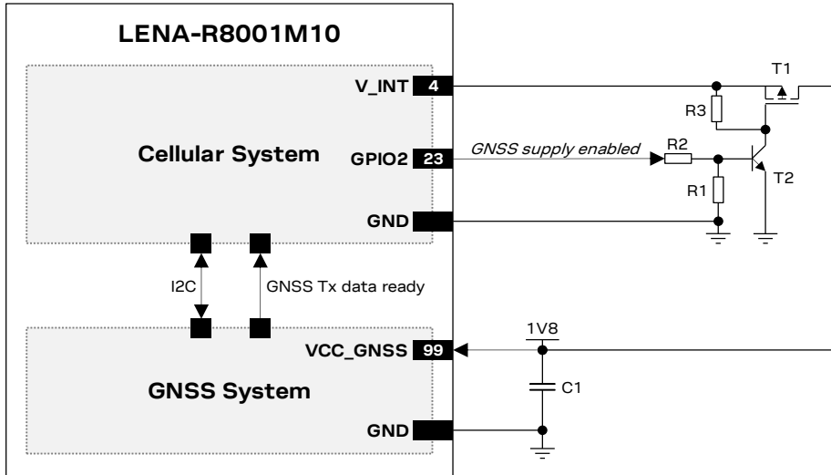
Figure 62: Application circuit for LENA-R8001M10 modules GNSS system supply using LENA-R8001M10 cellular system
