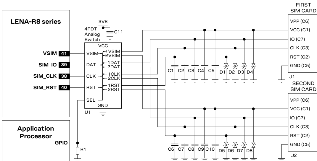
Figure 47: Application circuit for the connection to two removable SIM cards, with SIM detection not implemented
