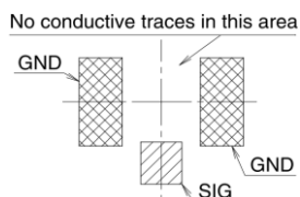
Figure 37: U.FL surface mounted connector mounting pattern layout
