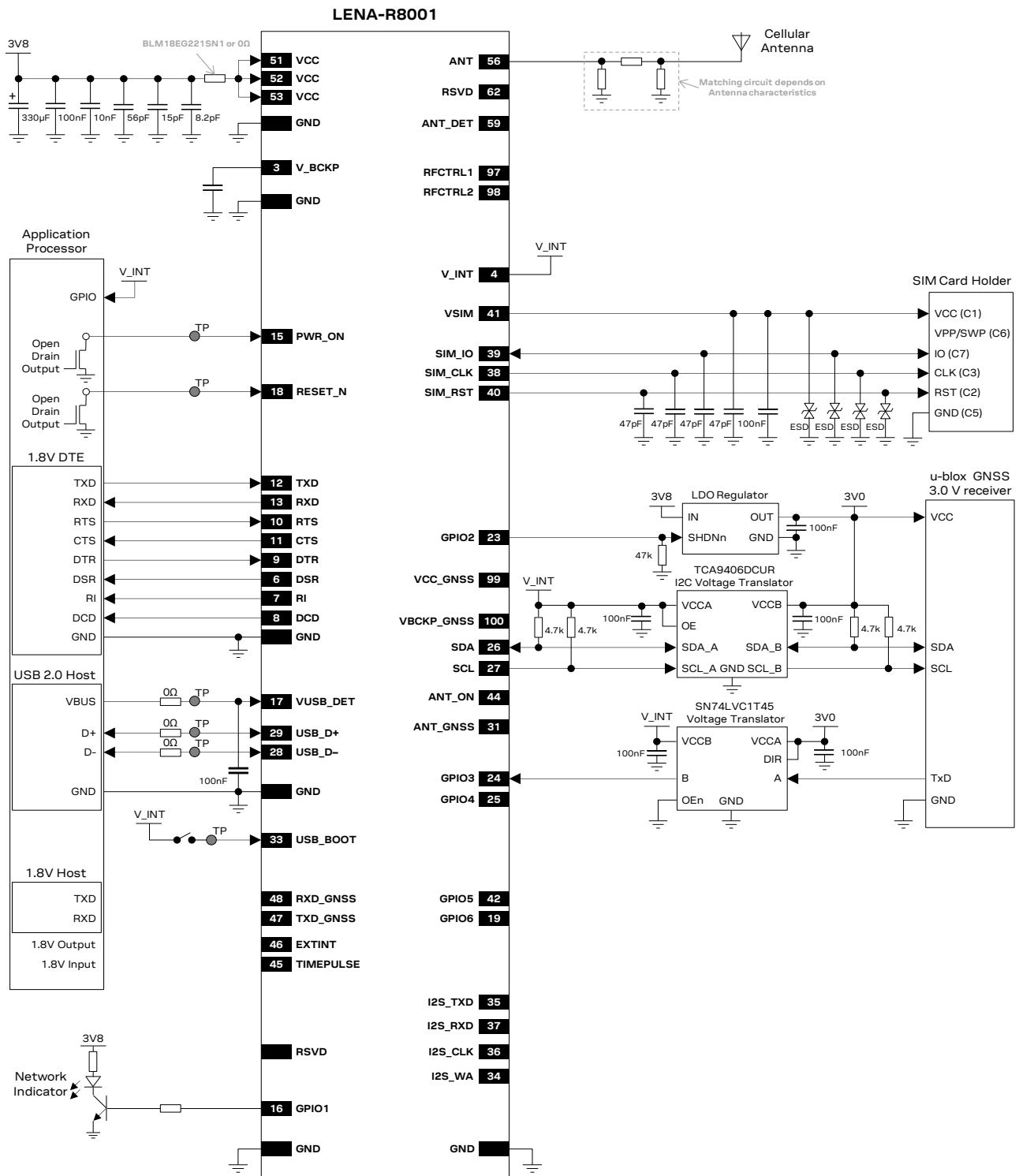
Figure 68: Illustrative example of schematic diagram to integrate a LENA-R8001 module using almost all interfaces
