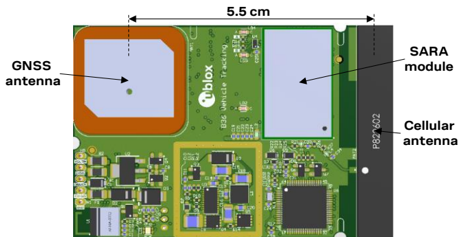
Figure 43: PCB top rendering for the u-blox B36 blueprint with annotated distance between cellular and GNSS antennas
