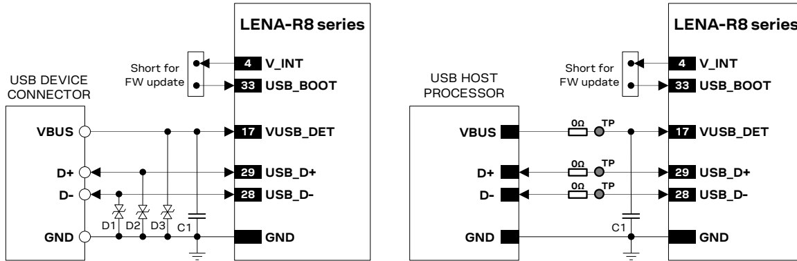
Figure 54: USB Interface application circuits
