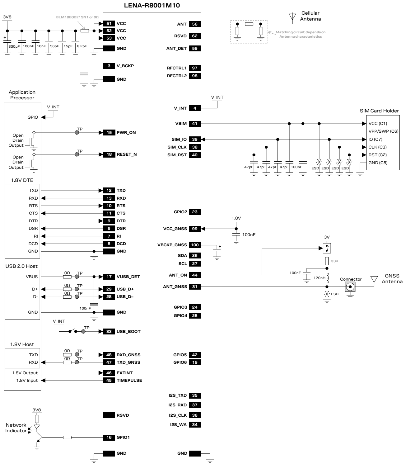
Figure 69: Illustrative example of schematic diagram to integrate a LENA-R8001M10 module using almost all interfaces
