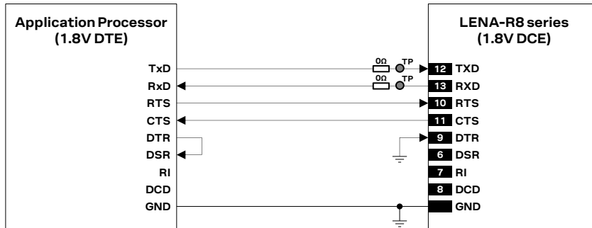
Figure 50: UART interface application circuit with partial V.24 link in the DTE/DCE serial communication (1.8 V DTE)
