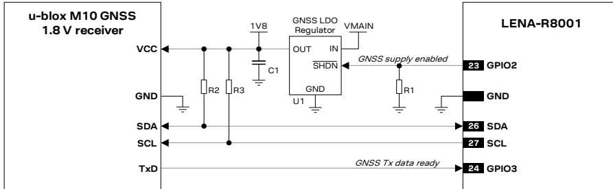
Figure 57: Application circuit for connecting LENA-R8001 modules to u-blox 1.8 V GNSS receivers
