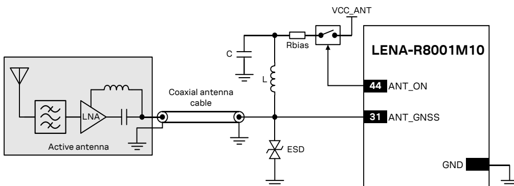
Figure 40: Typical circuit with active antenna connected to GNSS RF interface, using an external supply
