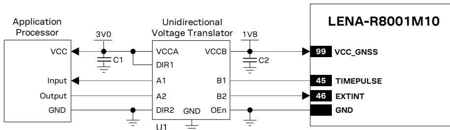
Figure 66: Application circuit for LENA-R8001M10 GNSS PIOs with 3 V external host application processor
