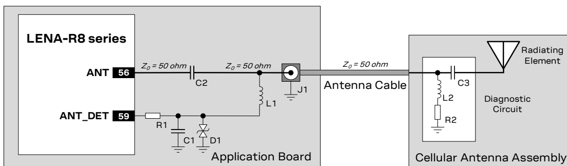
Figure 44: Suggested schematic for antenna detection circuit on application PCB and diagnostic circuit on antenna assembly
