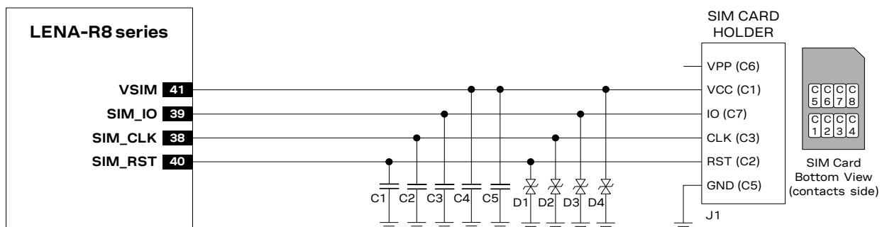
Figure 45: Application circuit for the connection to a single removable SIM card, with SIM detection not implemented
