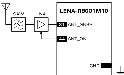
Figure 39: Typical circuit for GNSS passive antenna placed far away from the module
