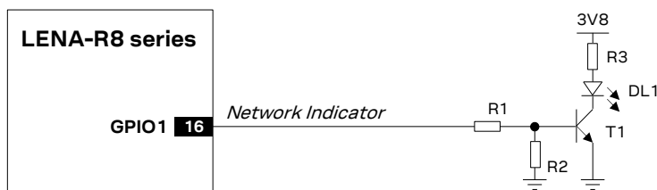
Figure 60: Application circuit for network indication provided over GPIO1
