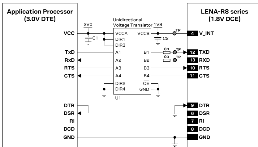
Figure 51: UART interface application circuit with partial V.24 link in DTE/DCE serial communication (3.0 V DTE)
