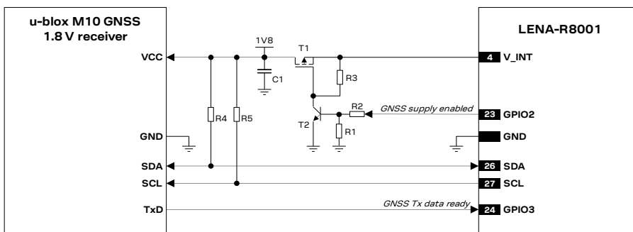
Figure 58: Application circuit for connecting LENA-R8001 modules to u-blox 1.8 V GNSS receivers using V_INT as supply
