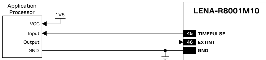
Figure 65: Application circuit for LENA-R8001M10 GNSS PIOs with 1.8 V external host application processor
