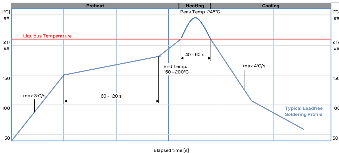
Figure 70: Recommended soldering profile
