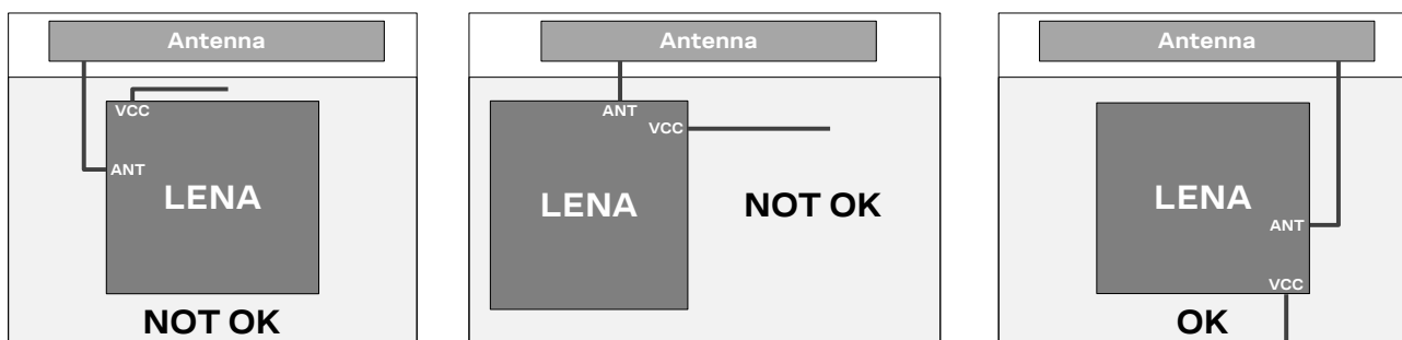
Figure 29: VCC line routing guideline for designs integrating an embedded antenna
