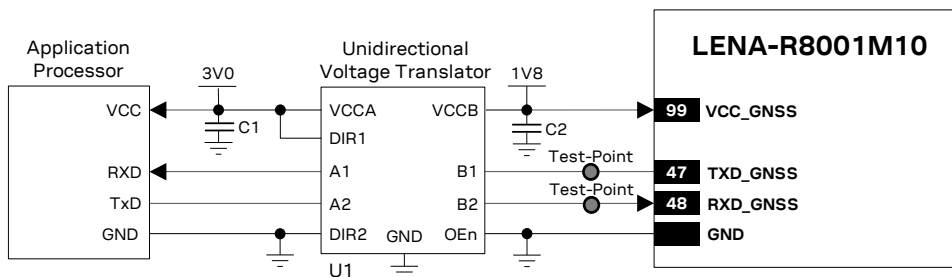
Figure 64: Application circuit for LENA-R8001M10 GNSS UART with 3 V external host application processor
