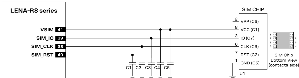
Figure 46: Application circuit for the connection to a single solderable SIM chip, with SIM detection not implemented
