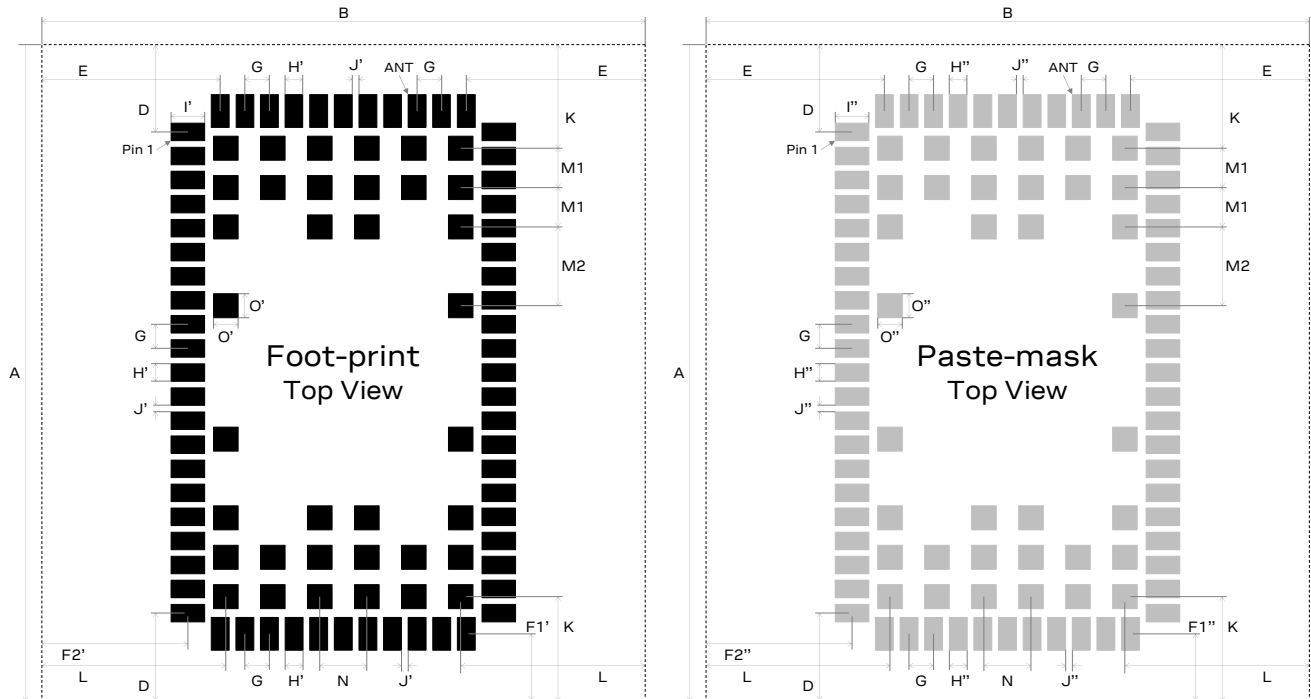
Figure 67: LENA-R8 series modules suggested footprint and paste mask (application board top view)
