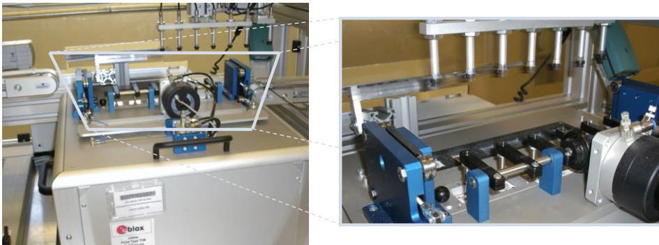
Figure 71: Automatic test equipment for module tests
