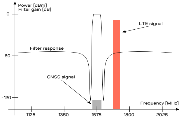
Figure 41: Interference due to transmission in LTE B3, B4 and B66 low channels (1710 MHz) adjacent to GNSS frequency range (1561 to 1605 MHz).
