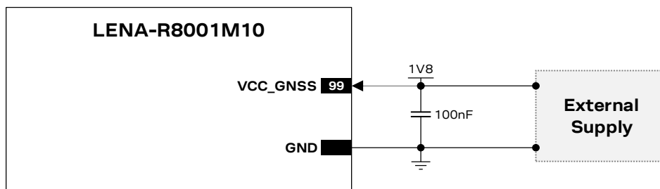
Figure 61: Application circuit for LENA-R8001M10 modules GNSS system supply using external 1.8 V supply system
