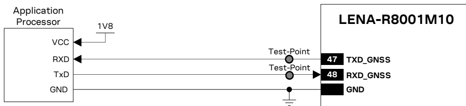
Figure 63: Application circuit for LENA-R8001M10 GNSS UART with 1.8 V external host application processor
