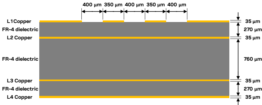
Figure 55: Example of USB line design, with Z_0 close to 90 \Omega and Z_{CM} close to 30 \Omega , for the described 4-layer board layout
