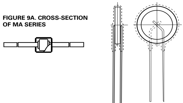
FIGURE 9B. CROSS-SECTION OF RADIAL LEAD PACKAGE
